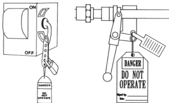
Figure 9 Examples of Lockout
