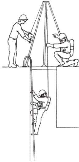
Figure 11 Entry With Hoist and Standby Personnel
