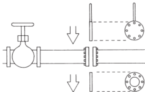
Figure 10 Method of Blanking Hydraulic/Pneumatic Lines
